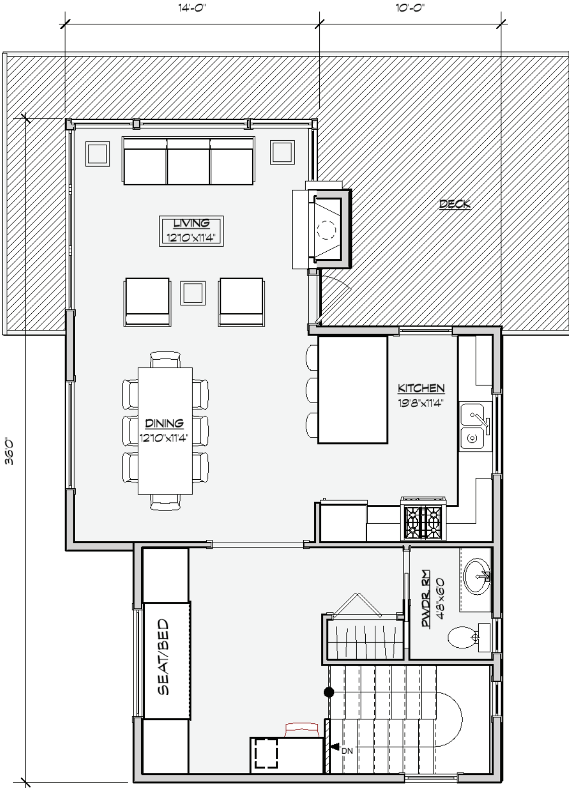
AVOCET SECOND FLOOR PLAN
