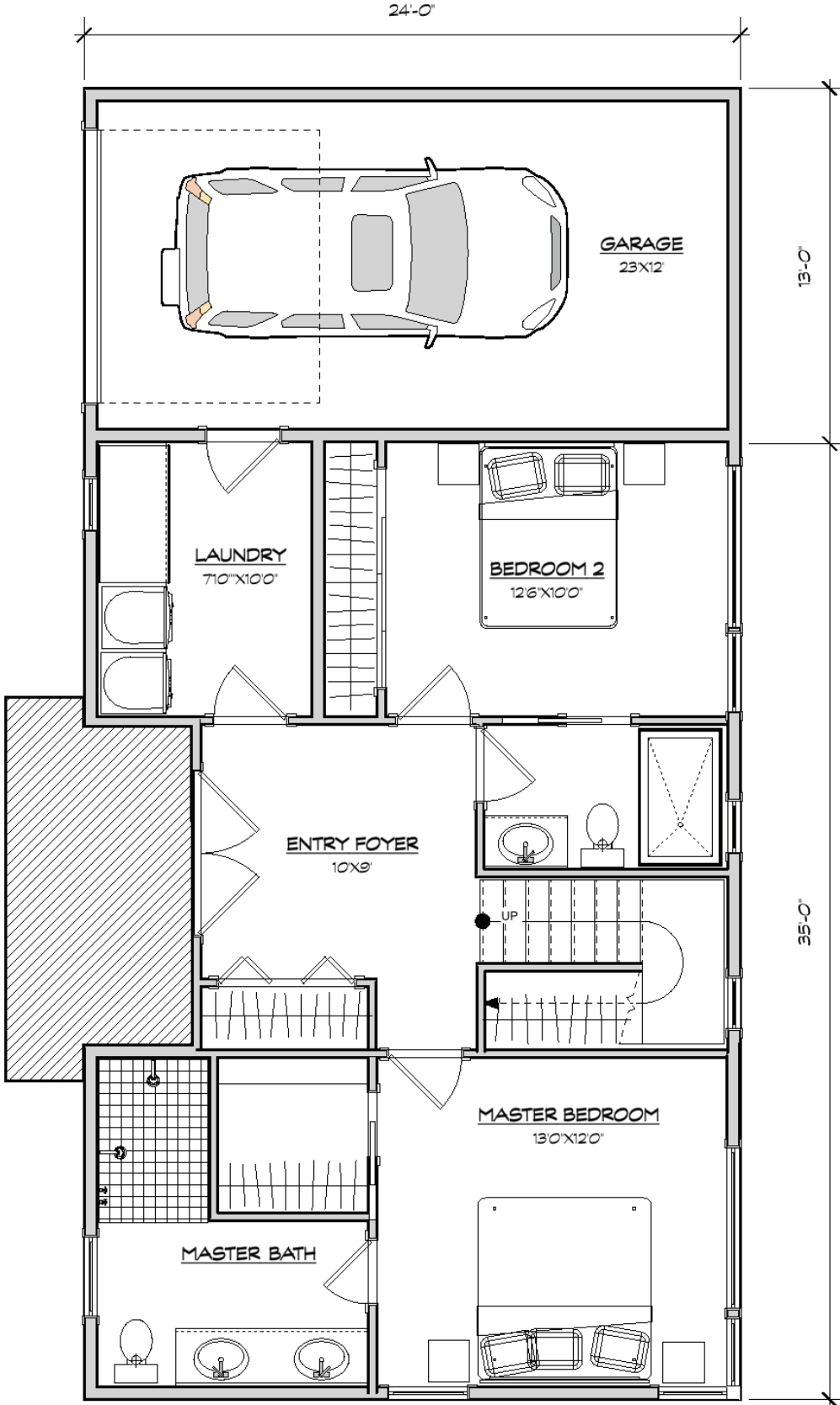
AVOCET FIRST FLOOR PLAN
